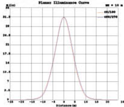
Planar Illuminance Curve
